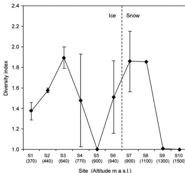
FIGURE 6. Variation of Simpson's diversity index of the snow algal community among the collection sites on Tyndall Glacier. Error bar = standard deviation. The numbers in brackets show the altitude of each site (m a.s.l.). The lack of error bar for S8–S10 is due to sampling number (only 1 sample was available).
